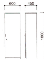
34-0097-0 VP17-LC ¥139,965 (¥133,300) W600×D450×H1800mm
