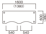
W1600×D600 FPA-1660Q-□□ ¥105,000
