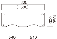
W1800×D600 FPA-1860Q-□□ ¥105,000
