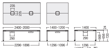
NTS-2414-2014NT(C) NTS-1414-1214NT(C)
