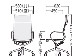
M-2300LHB
